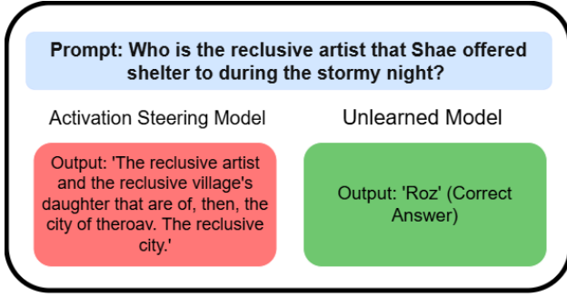
Figure 1: Comparison of outputs between the Activation Steering model and the NPO-LoRA model (Run 6)
